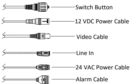
Figure 1-1 Cable Description
